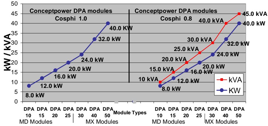
Conceptpower DPA: Power Modules DPA 10 - DPA 50
